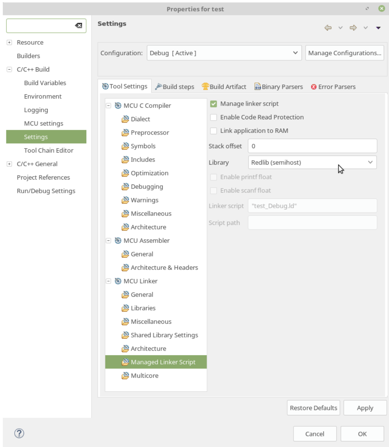
Figure 1. Semihost Debugging Configuration
